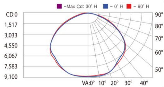
< Asymmetric Wide 130° >
