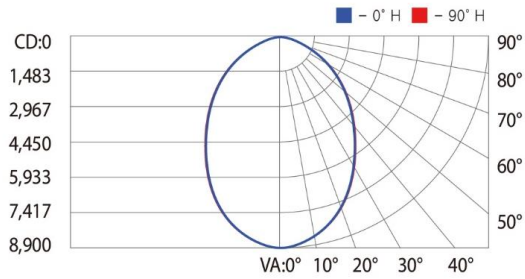
< Asymmetric Wide 90° >
