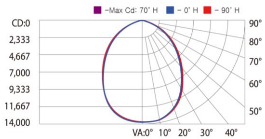
< Asymmetric Wide 90° >
