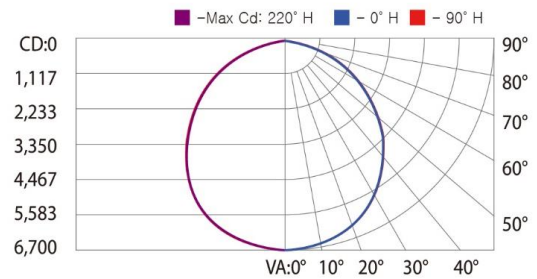
< Asymmetric Wide 130° >
